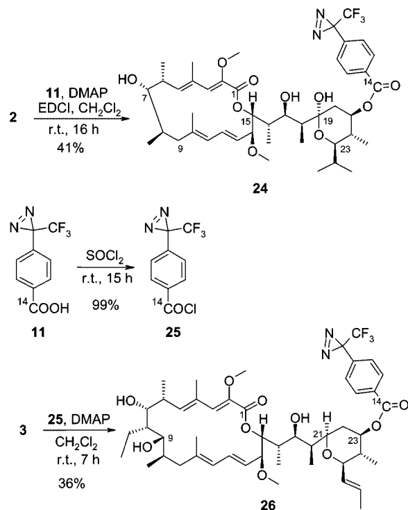
Scheme 3. Coupling reaction of diazirine 11 with ATPase inhibitors 2 and 3 .
