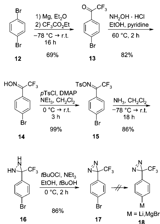
Scheme 1. Synthesis of p -bromophenyldiazirine 17 .
