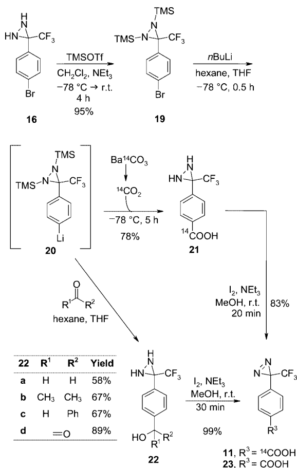
Scheme 2. Completion of the synthesis.
