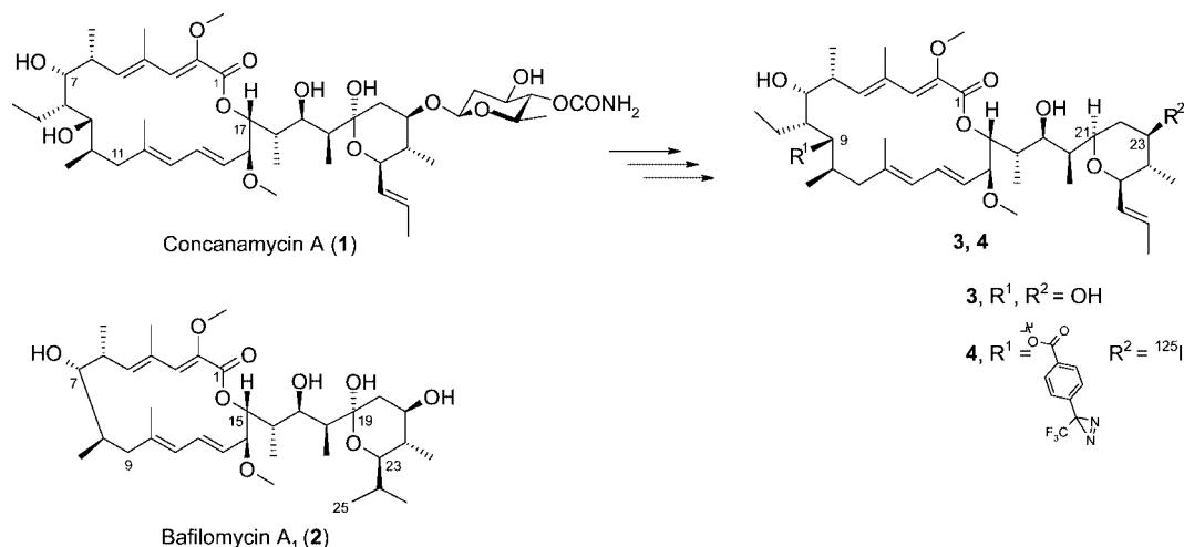
Figure 1. Structures of concanamycin A (1), bafilomycin A 1 (2), and concanolides 3 and 4.
